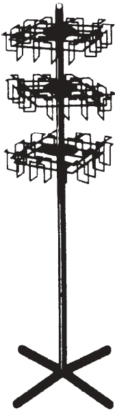
4566 4340 base 4341 upright 3- 4342 6 pocket tiers 4352 sign holder • tiers should be 9" apart
