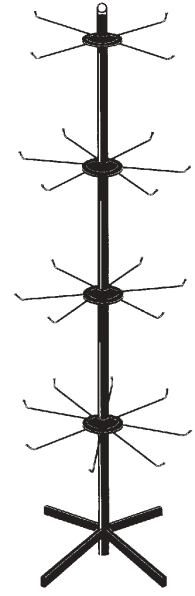
4570 4340 base 4341 upright 4353 tier 2- 4354 tiers 4355 tier 4352 sign holder
